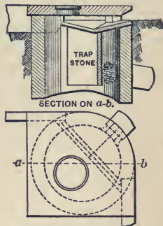
FIG. 5. STONE TOP INLET WITH CATCH-BASIN.
